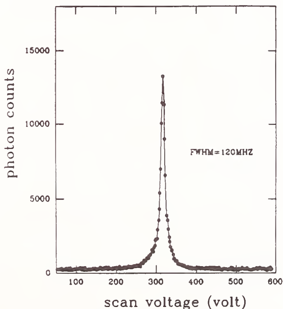
Fig. 2. Ar II 3d' 2G_{9/2} - 4p' 2F^0_{7/2} resonance spectrum.
